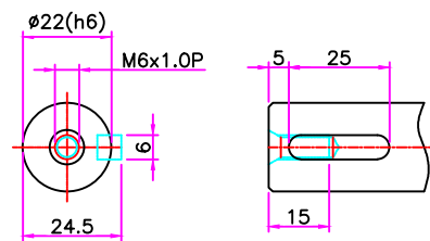
Shaft Option 1(K)
