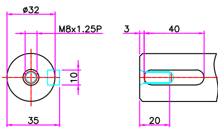
Shaft Option 1(K)
